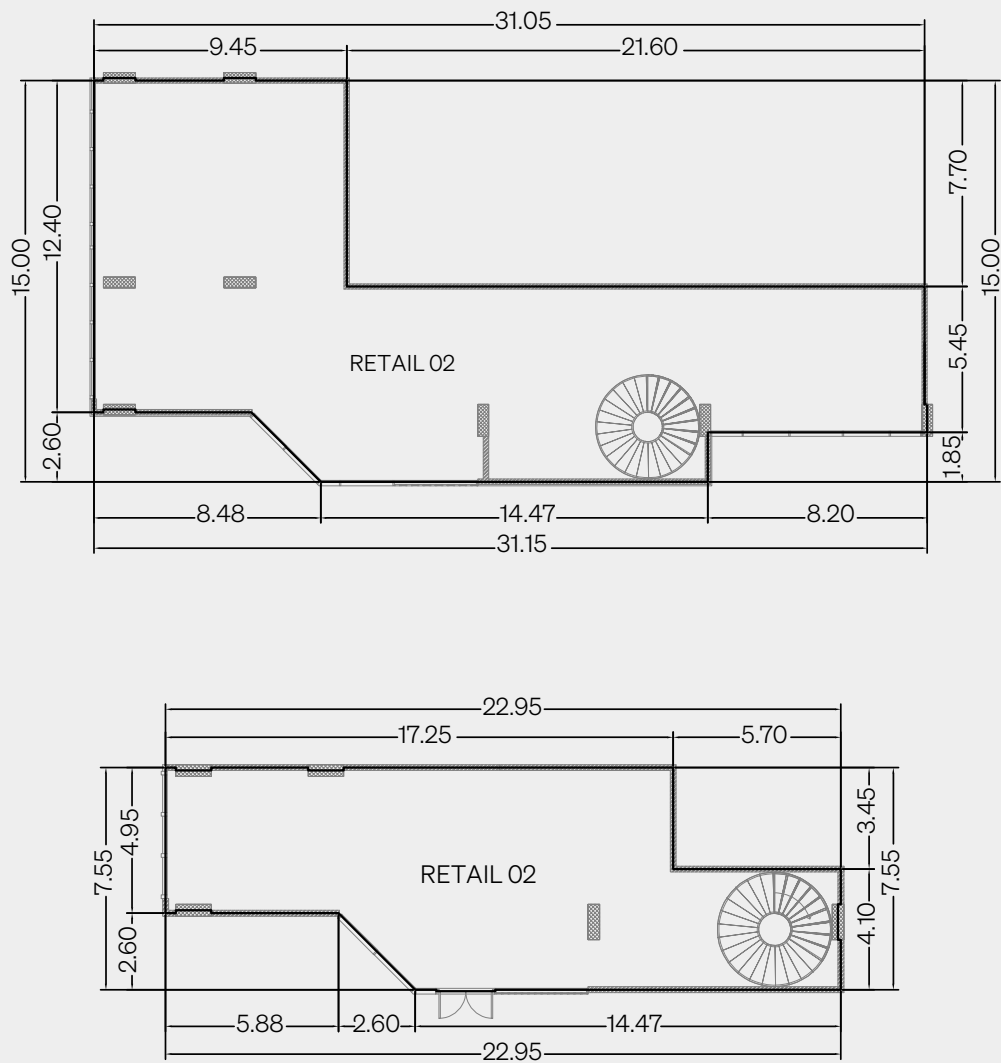
UNIT DETAIL SCALE: NTS
