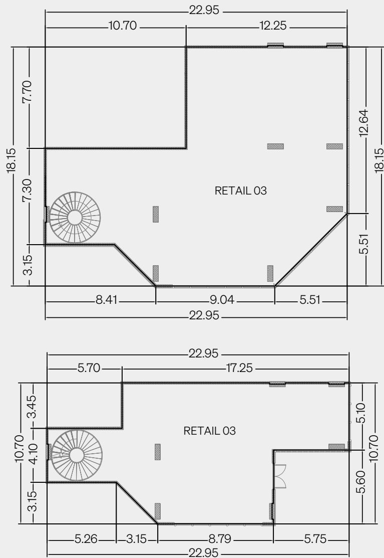
UNIT DETAIL SCALE: NTS
