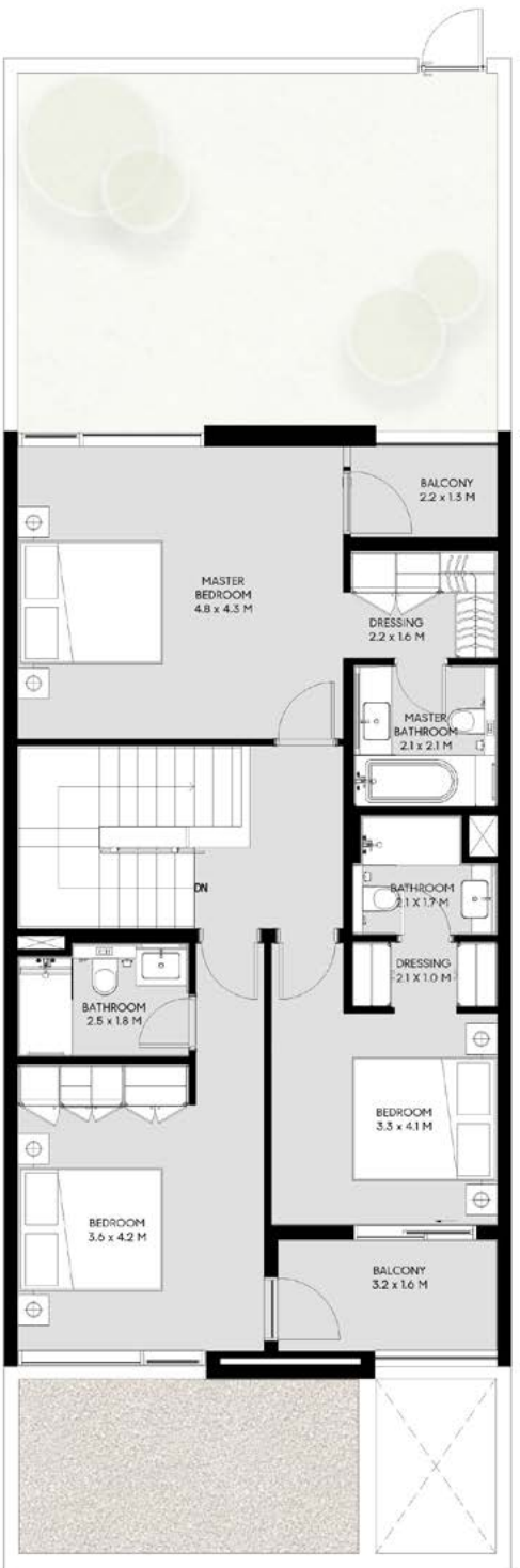
First Floor
