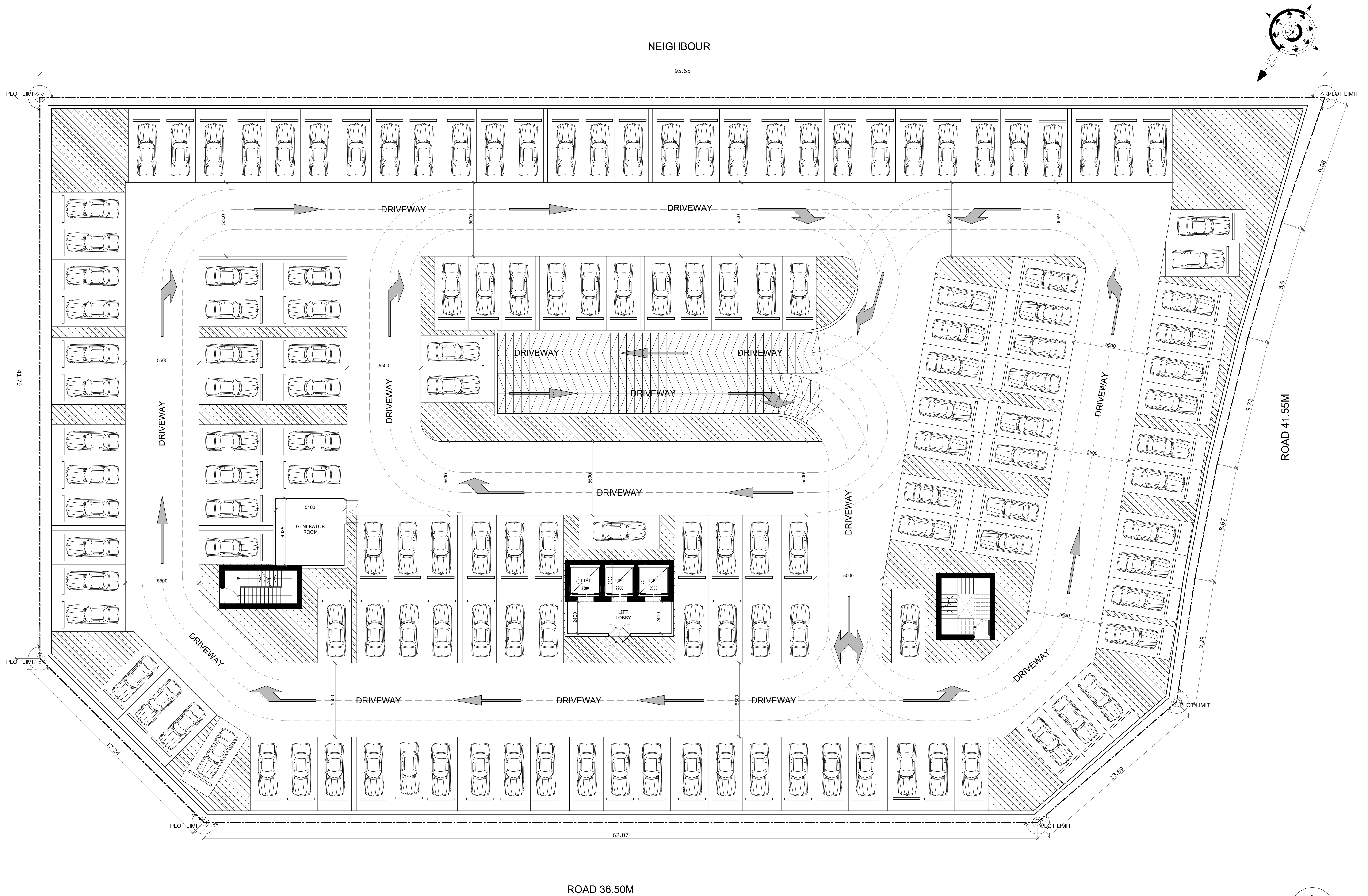
BASEMENT FLOOR PLAN 1 TOTAL NO.OF PARKING - 147 NO.S
