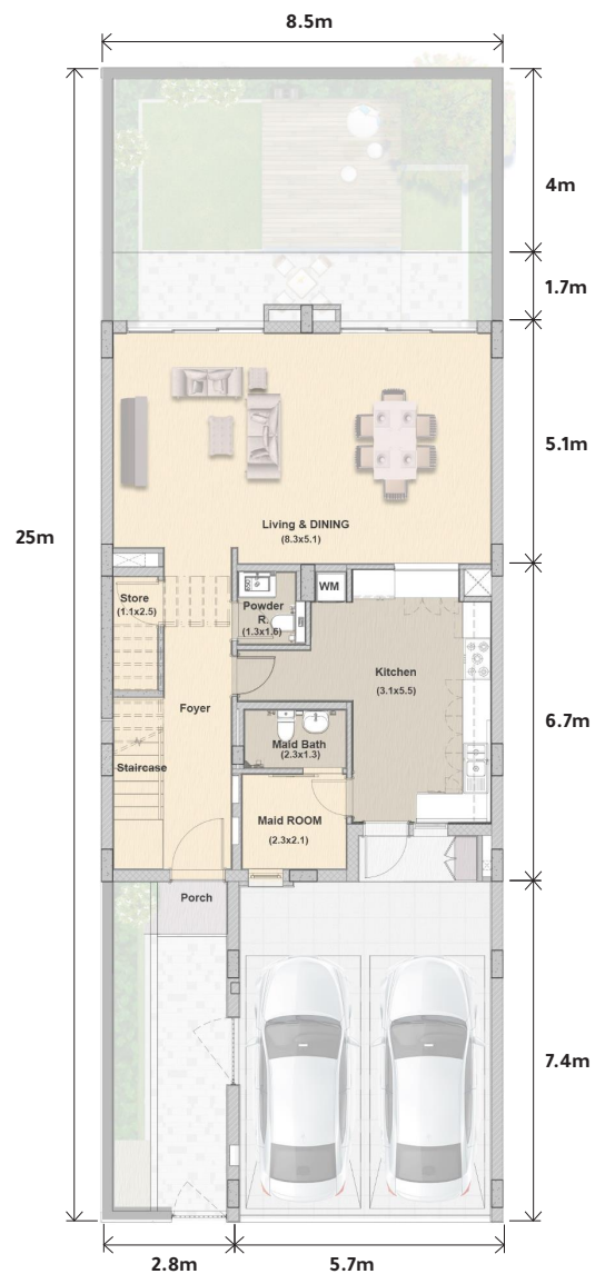
GROUND FLOOR LAYOUT
