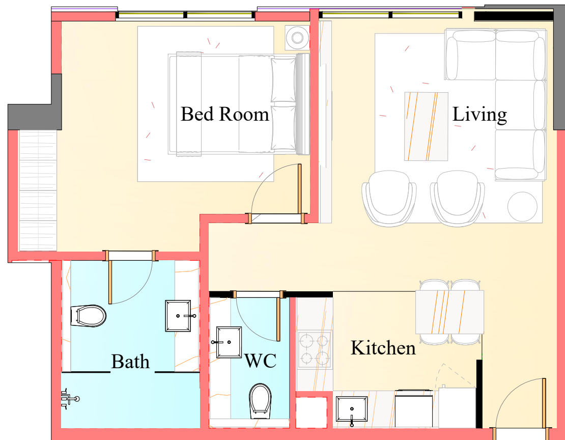
APARTMENT LAYOUT
