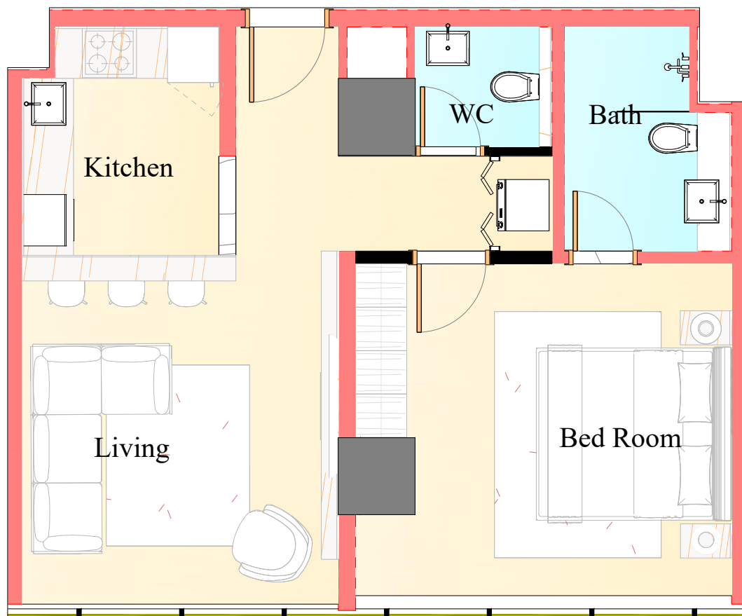
APARTMENT LAYOUT
