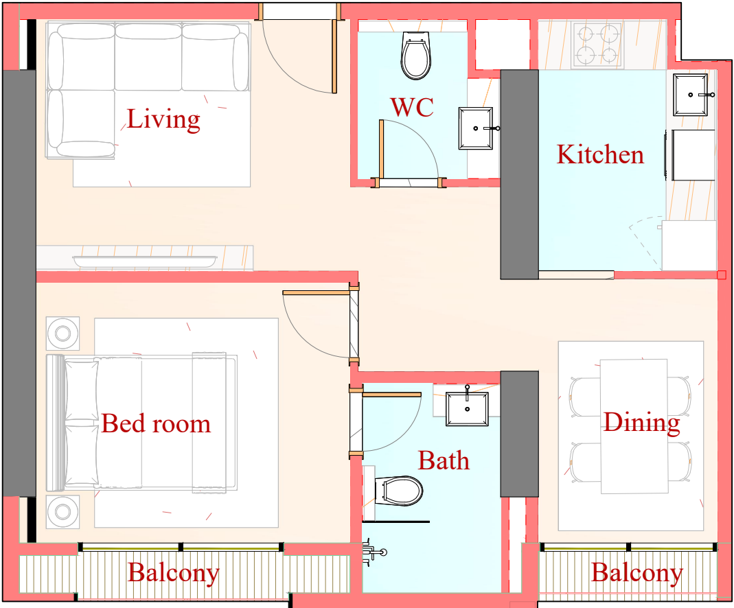
APARTMENT LAYOUT
