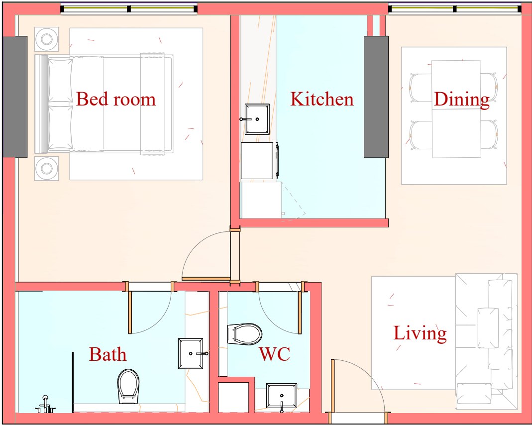
APARTMENT LAYOUT
