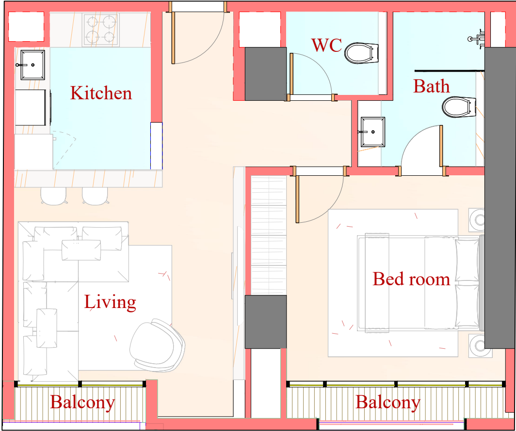
APARTMENT LAYOUT
