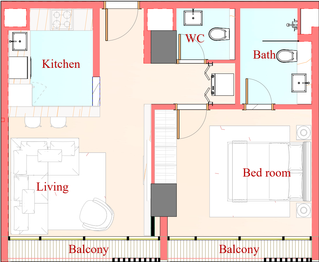
APARTMENT LAYOUT
