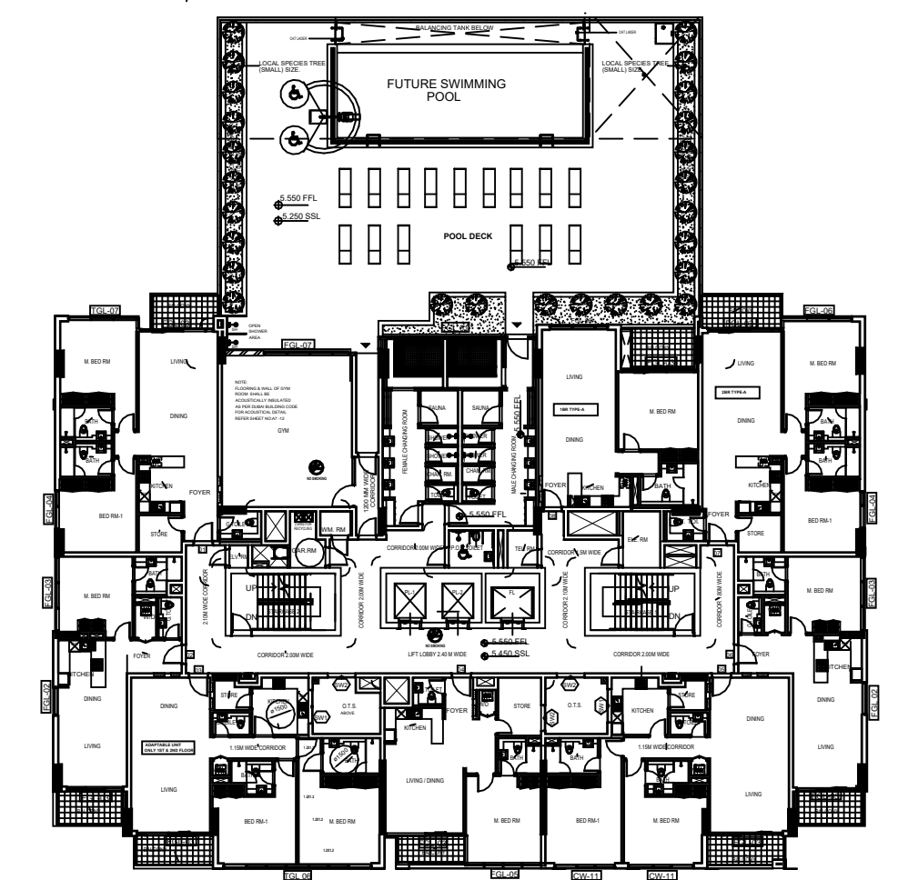
1ST FLOOR
