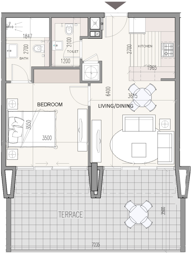
1-BEDROOM - FOURTH FLOOR
