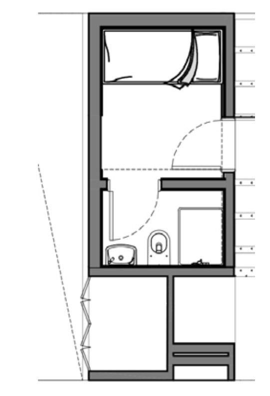
DRIVER ROOM (OPTIONAL PROVISION)
