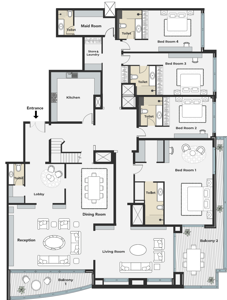
FLOOR PLAN
