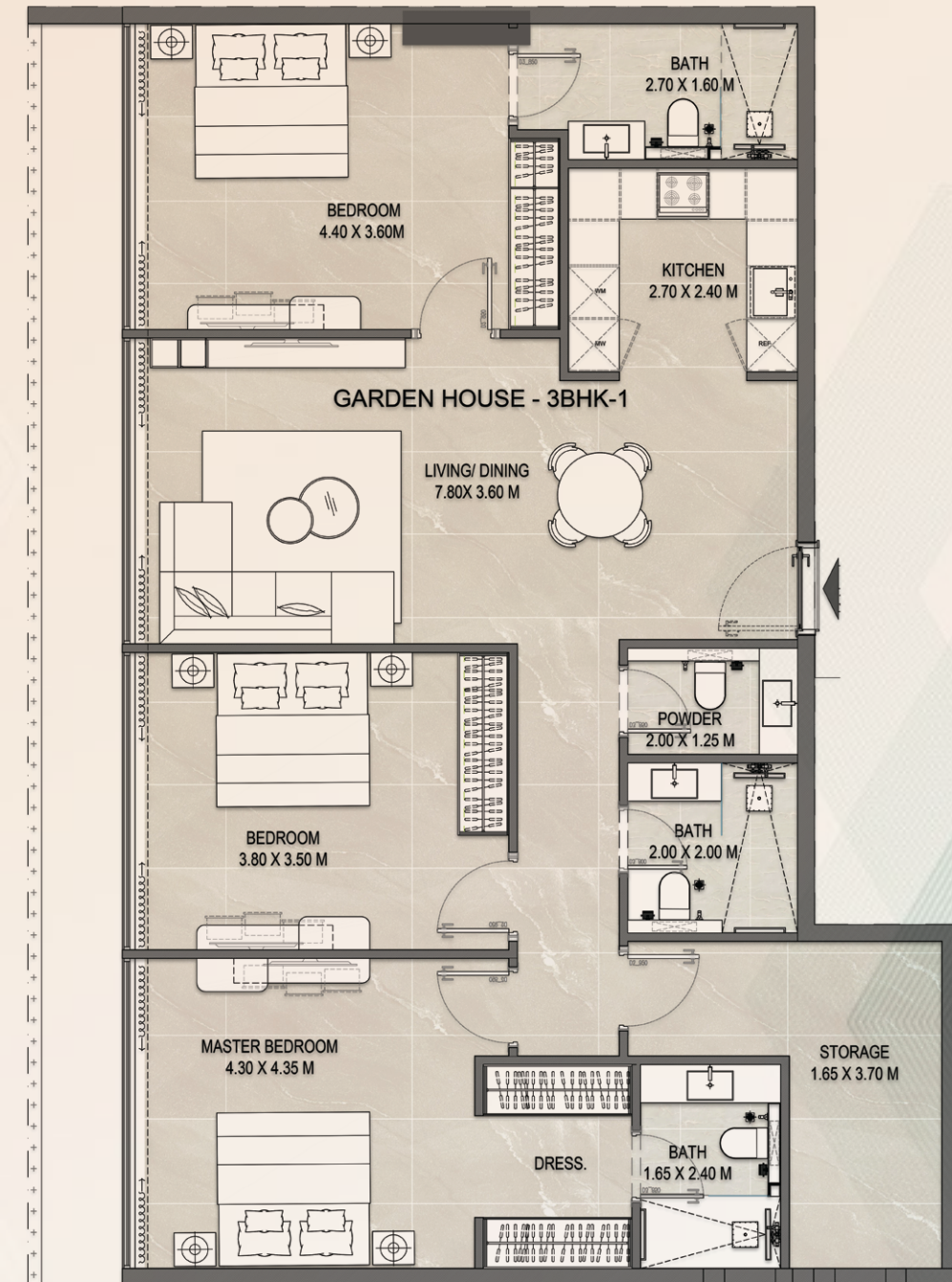
01 GARDEN HOUSE 3BHK-1 SCALE 1:100@A1
