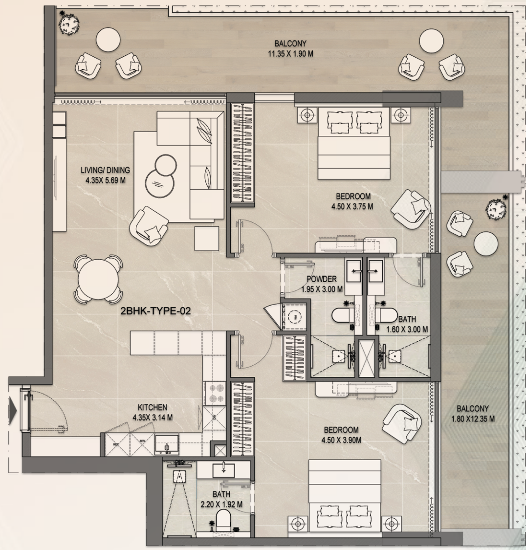
01 2BHK TYPE-02 FURNITURE PLAN SCALE 1:100@A1
