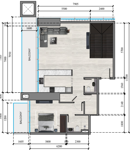
GROUND FLOOR LEVEL
