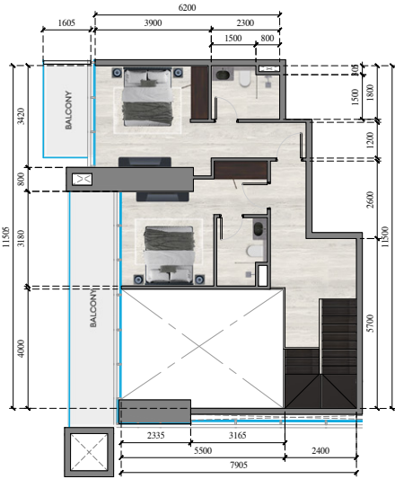
FIRST FLOOR LEVEL
