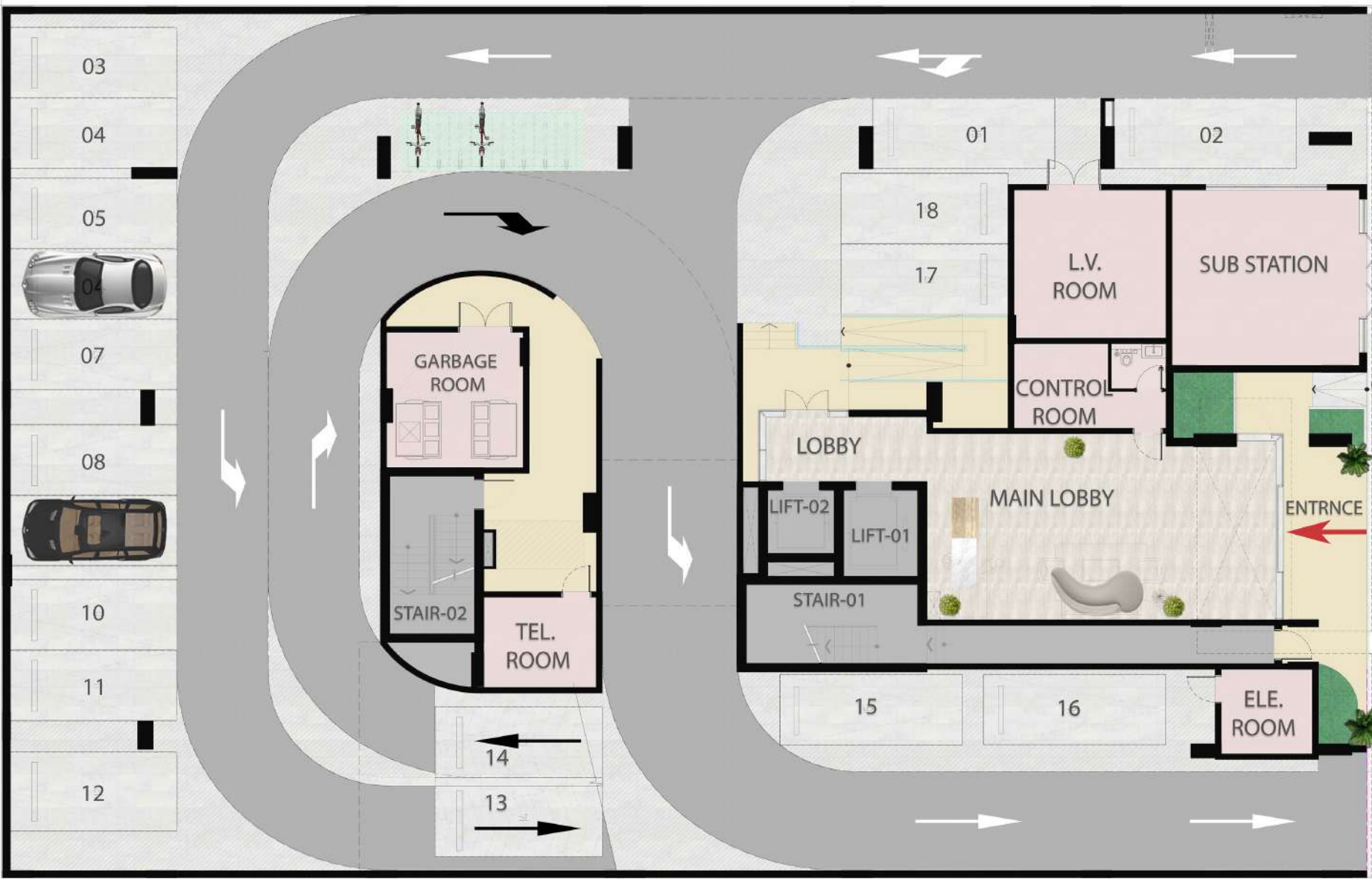
GROUND FLOOR
